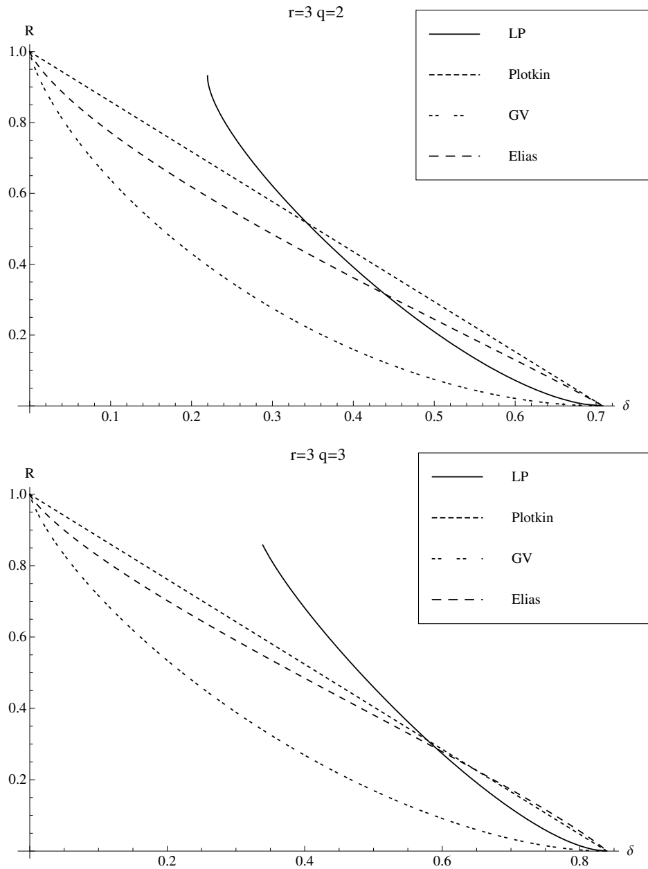
Figure 5.3: Bounds on codes for r = 3 .
