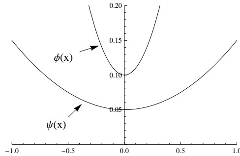
Figure 7.2: An example illustrating Lemma 7.9. Here \phi(x) = x^2 + 0.1 , \psi(x) = 0.1x^2 + 0.05 , S = [-1, 1] . All the functions \phi(x), \psi(x), \phi(x) - \psi(x) , and \phi(x)/\psi(x) attain their minimum at x = 0 .
