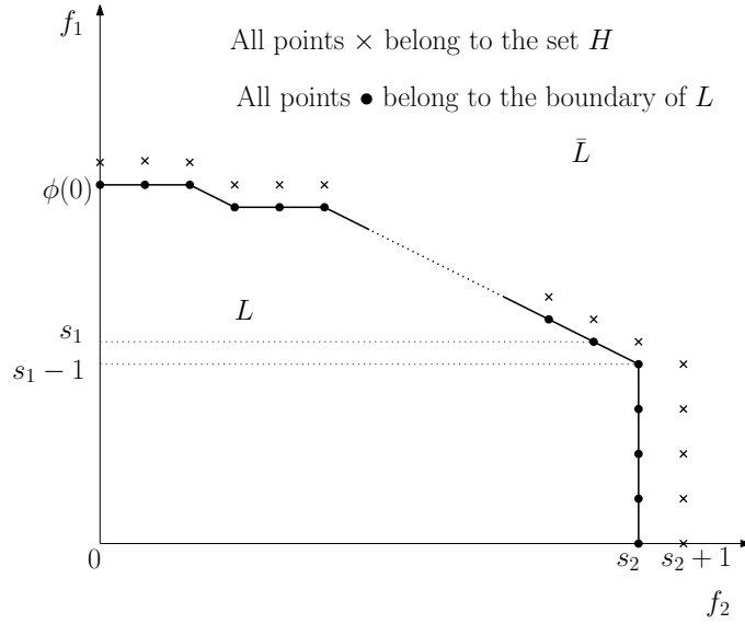
Figure 5.1: The region L
