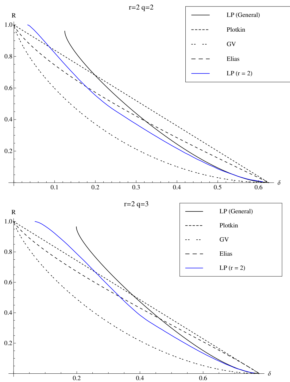
Figure 5.2: Bounds on codes for r = 2 .
